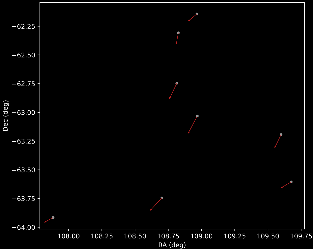
GALAH DR4 Cluster 6 Proper Motion Vectors (n=8)
