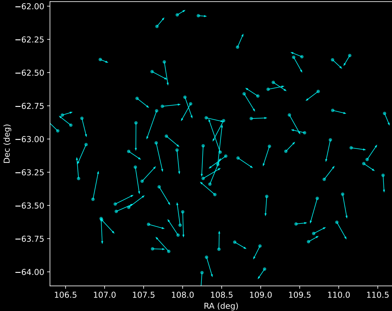
GALAH DR4 Noise Stream Proper Motion Vectors (n=83)
