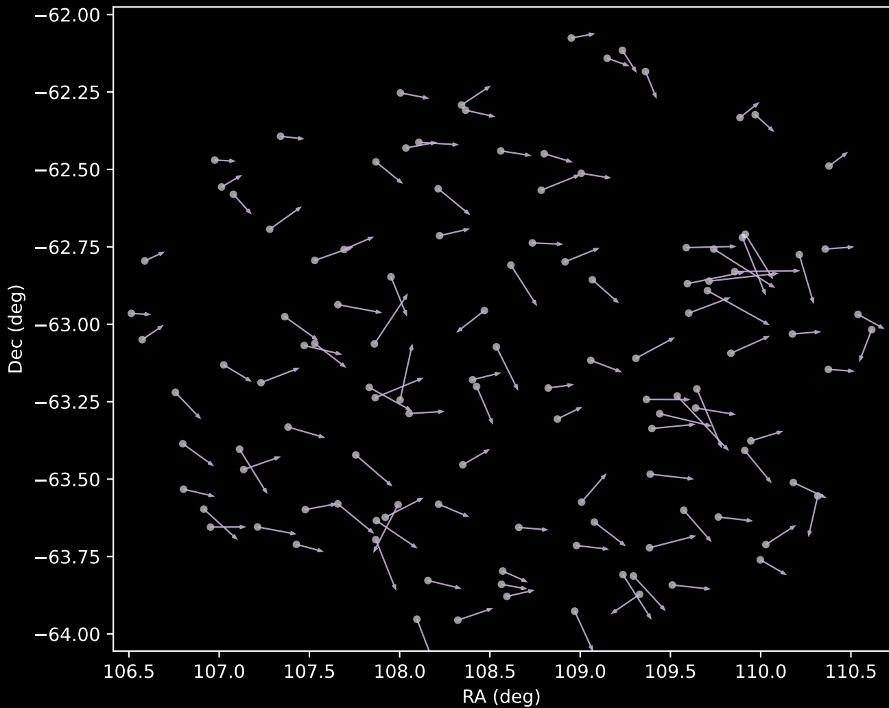
GALAH DR4 Cluster 9 Proper Motion Vectors (n=119)
