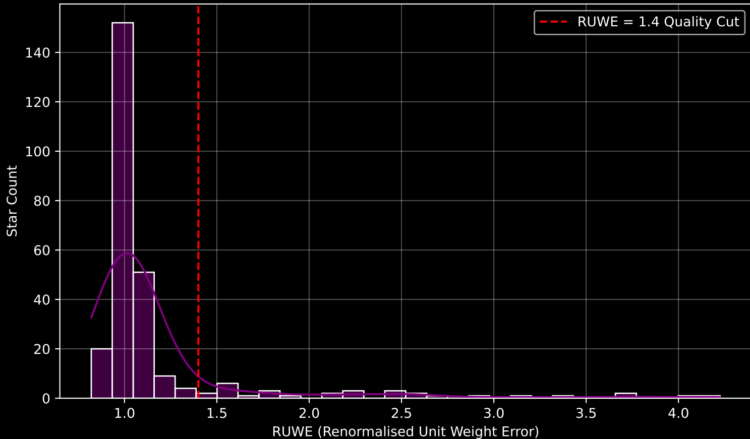
GALAH DR4 Field [6928] RUWE Distribution (n= 267)
