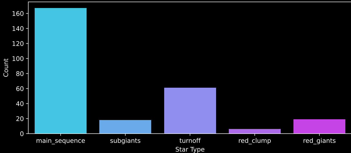
GALAH DR4 Field: [6928] Count plot of Star Type
