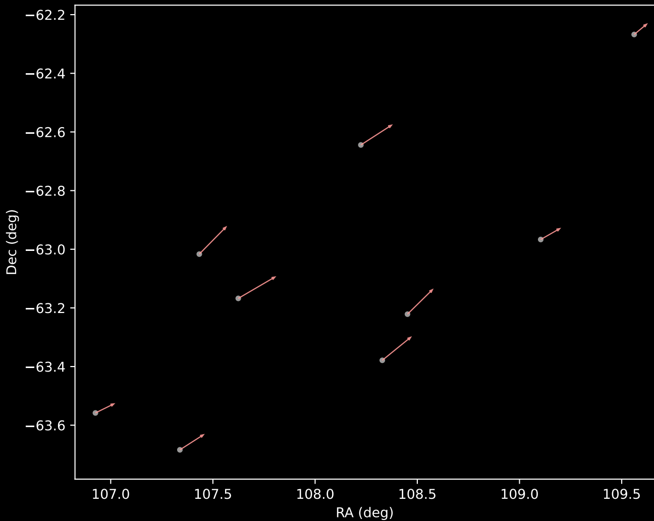
GALAH DR4 Cluster 7 Proper Motion Vectors (n=9)
