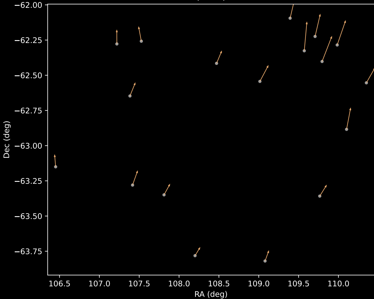
GALAH DR4 Cluster 3 Proper Motion Vectors (n=18)
